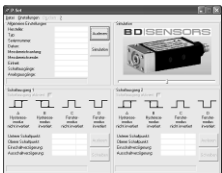
Fig. 2 Programming software
